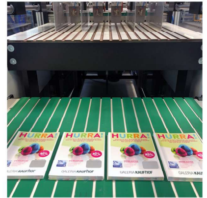
Discharging the stacks via conveyor belt. Interface to following machine or removal by hand
