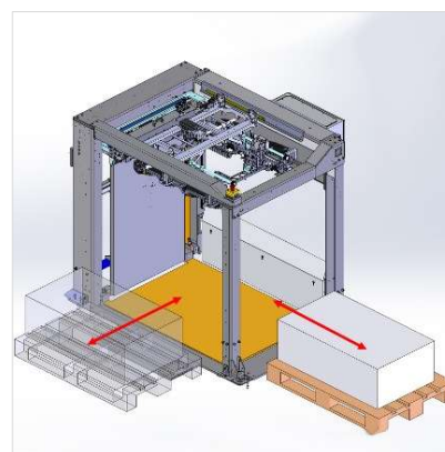
4) Side and rear loading
