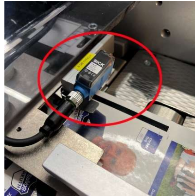
7) Print mark sensor in production direction
