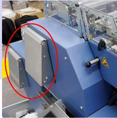
11) Ejection unit for incomplete decks
