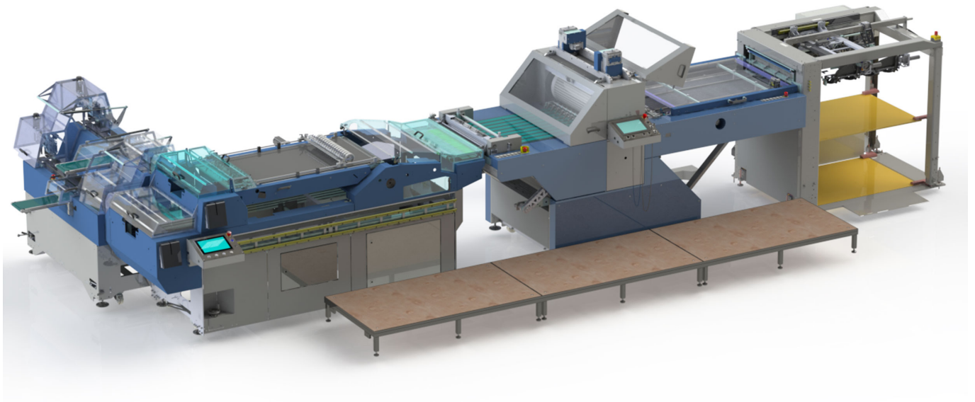
Automated Playing Card Production System consisting of a BOGRAMA BSR 750 rotary die-cutting machine and an ACC 750 DHS Automatic Card Collator and Stacker.
