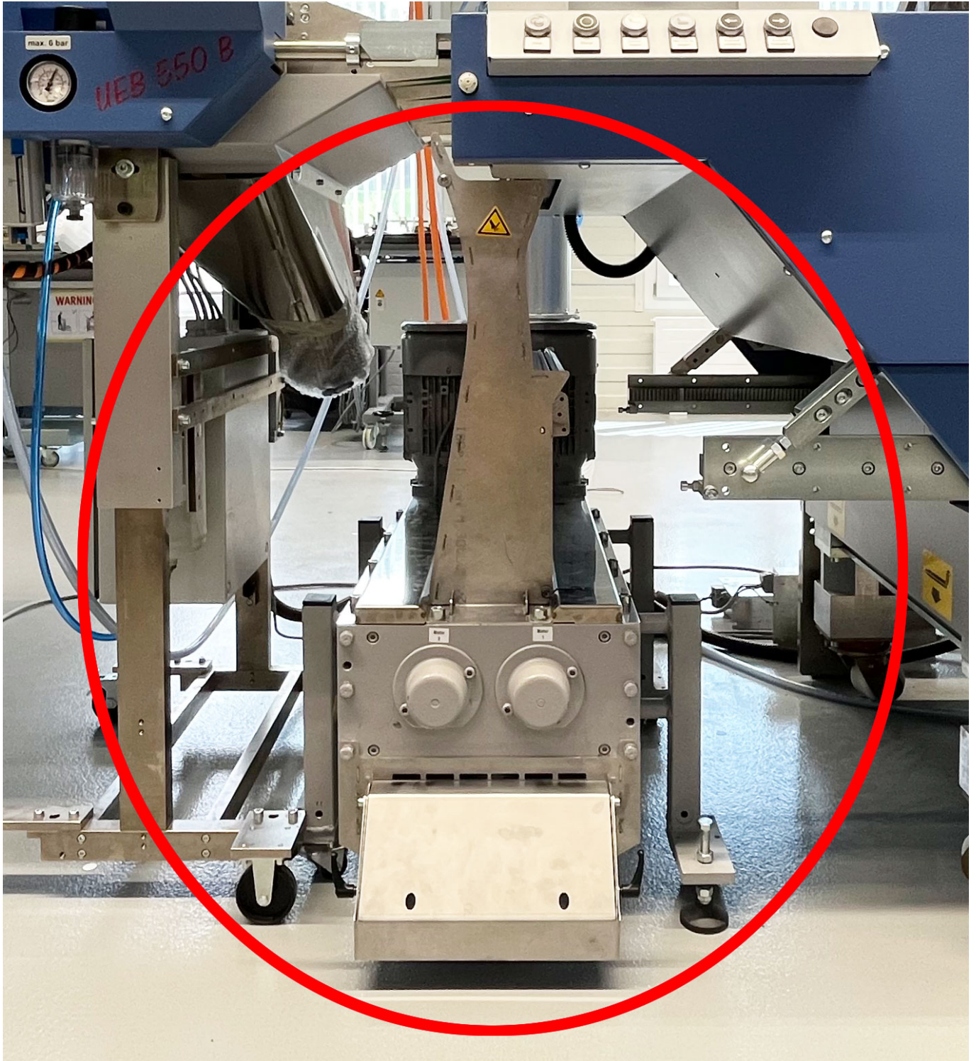
Punch grid shredder for BSR 550 Servo Rotary die-cutter with flat pile or pallet feeder.
