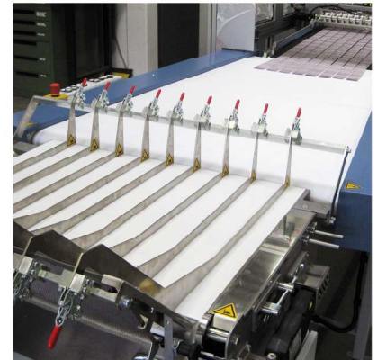
Delivery variant spreading belt with SB 810 Shaft delivery
